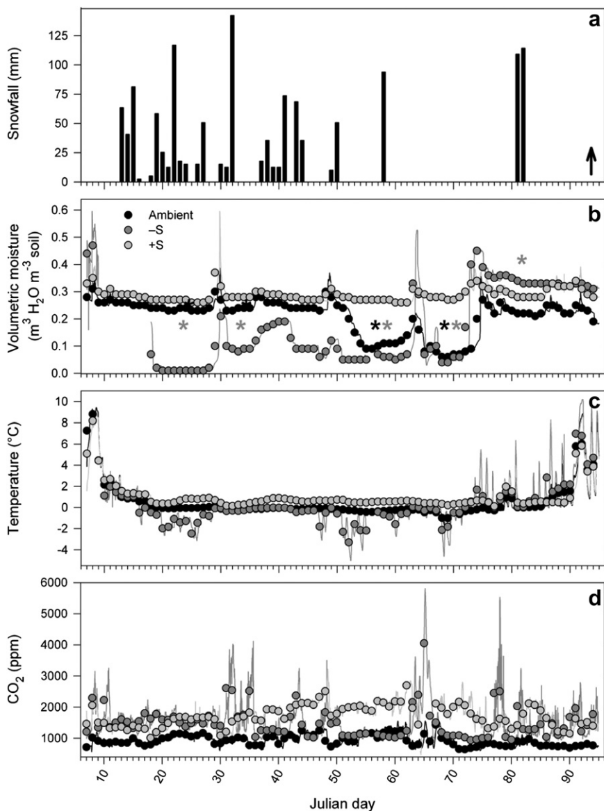
Fig. 1. Snowfall events (vertical bars in a ) and the effects of snow manipulations on soil moisture ( b ), temperature ( c ), and \text{CO}_2 concentration ( d ). Treatments included an ambient snowfall (Ambient), snow removal ( -S ), and snow addition ( +S ). The solid lines in b , c , and d represent real-time sensor data that was generated every 10 s and averaged to create a 30 min value. Circles in b , c , and d represent the daily means of these data that were used in our time-series regression analyses to quantify respiration sensitivity. Lines and circles are color-coded (ambient snowfall = black, snow removal = dark gray, and snow addition = light gray). \text{CO}_2 values were measured at a depth of 2 cm and soil moisture and temperature were measured over depth of 0–5 cm. Asterisks in b indicate a freeze–thaw cycle (FTC) in the ambient (black) and or -S treatments (dark gray); there were no FTCs in the +S treatment. An upward pointing arrow in a identifies the date (April 3rd, Julian day = 94) for the bacterial community analysis during spring–thaw. Data from days 3–12 in the -S were removed due to a malfunction with the \text{CO}_2 sensor.
