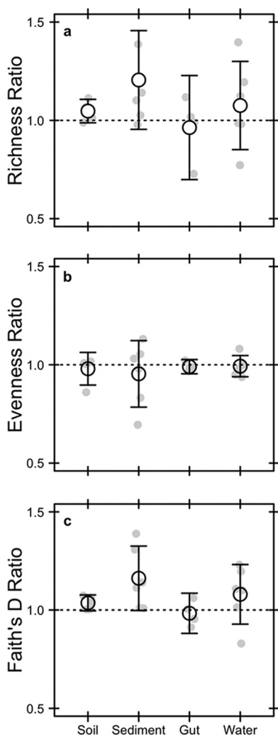
FIG 3 Effect of relic DNA on within-sample (alpha) bacterial diversity in different ecosystem types. We tested for the effects of bias caused by relic DNA by calculating diversity ratios for richness (a), evenness (b), and phylogenetic diversity (c). The ratios reflect the diversity of the total DNA pool (intact + relic) divided by the diversity of the intact DNA pool. Relic DNA did not bias any measures of diversity in any of the ecosystem types. Richness was calculated as the number of operational taxonomic units (97% sequence similarity of the 16S rRNA gene), evenness was calculated using Simpson's evenness index, and phylogenetic diversity was calculated using Faith's D index. Gray symbols are the observed data, and black symbols represent means \pm 95% confidence intervals.
