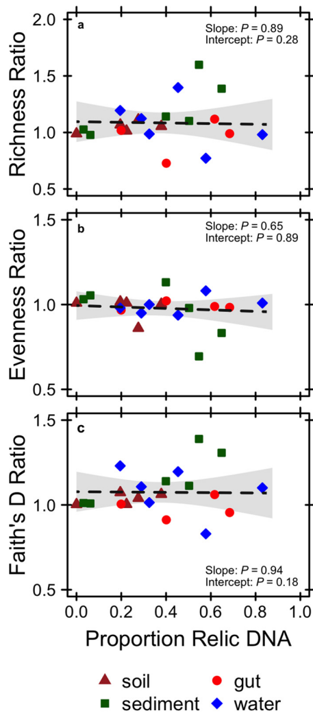
FIG 4 Linear regressions testing for the effect of relic DNA on measures of alpha-diversity. See the text for descriptions of how diversity metrics and diversity ratios were calculated. When included in the regression model as an indicator variable, ecosystem type had no effect on the slopes or intercepts of the regressions ( P \geq 0.26 ).
