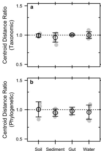
FIG 5 Effect of relic DNA on the among-sample (beta) bacterial diversity in different ecosystem types. (a and b) We tested for the effects of bias caused by relic DNA by calculating a beta-diversity ratio based on centroid distances. Centroid distances were estimated after performing principal-coordinate analyses (PCoAs) using taxonomic (a) and phylogenetic (b) distance metrics (Bray-Curtis and UniFrac, respectively). The centroid distance ratio was calculated on each sample within an ecosystem type and reflects the composition of the total DNA pool (intact + relic) relative to the intact DNA pool. Relic DNA had no effect on beta-diversity for any of the ecosystem types sampled. Gray symbols are the observed data, and black symbols represent means \pm 95% confidence intervals.
