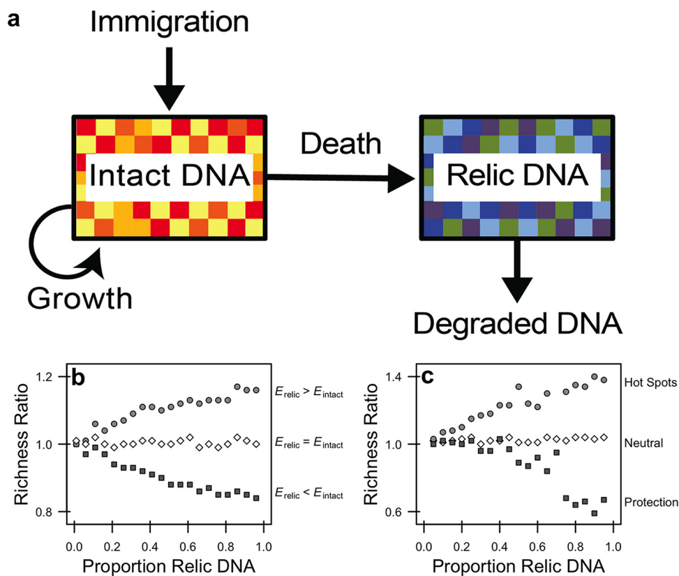
FIG 1 Modeling relic DNA dynamics. (a) The amount of relic DNA in a microbial environment is determined by inputs associated with the mortality of viable individuals with intact DNA and by losses associated with the degradation of relic DNA. If the diversity of sequences contained in the relic DNA pool is sufficiently different from that in the intact DNA pool, then relic DNA may bias estimates of microbial biodiversity (as indicated by different colored boxes) when sampling from the total (intact + relic) DNA pool. (b) We developed a sampling-based simulation model to explore the effects of mixing intact and relic DNA on estimates of diversity. We populated intact and relic communities with individuals from a lognormal species abundance distribution (SAD). We altered the diversity (i.e., evenness, E ) of the relic community by changing the scale parameter of the lognormal distribution describing the SAD. We then sampled and mixed the intact and relic communities so that the relic contribution to total community ranged from 0.01 to 0.96. (c) To gain mechanistic insight into how bias arises, we created a stochastic process-based model that captures features that influence relic DNA dynamics, including immigration, birth, death, and degradation (a). We simulated a range of degradation rates to achieve relic DNA pool sizes with proportions ranging between 0.05 and 0.95. To explore how degradation alters the SAD of the relic community, we explored three scenarios. First, we simulated a neutral scenario where relic DNA sequences produced by different species degrade at the same rate. Second, we simulated conditions under which physical, chemical, or biological processes reduce the degradation rate of relic DNA belonging to some species via protection. Third, we simulated “hot spots” where more abundant relic DNA sequences experience higher rates of relic DNA degradation, a condition that may arise in structured habitats where there are patchy distributions of individuals and their metabolic products (i.e., enzymes). We ran simulations for 10,000 time steps and then sampled the intact and relic communities. To quantify bias in diversity (b and c), we calculated “richness ratios” which reflect the number of species in the total DNA pool (intact + relic) divided by the number of species in the intact DNA pool in a simulation. When values for richness ratios equal 1, relic DNA has no effect on estimates of diversity; when richness ratios are >1 , relic DNA overestimates true diversity; and when richness ratios are <1 , relic DNA underestimates true diversity.
